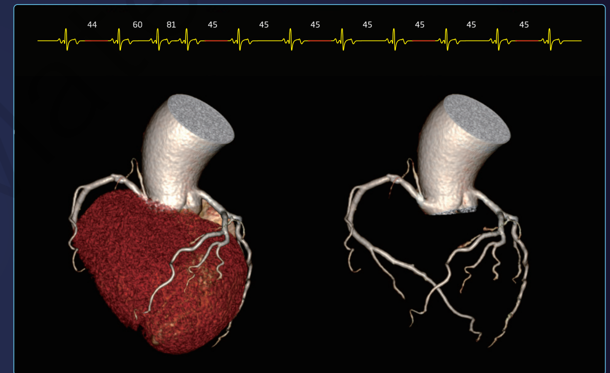
Arrhythmia Handling
