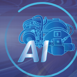
AI Adjustment
